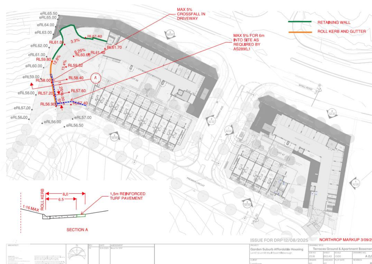
Figure 3-4 – Civil concept plans – Lot 67 and 68
