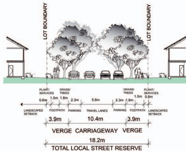
Section - Local Street with inset parking bays (optional raingardens)
