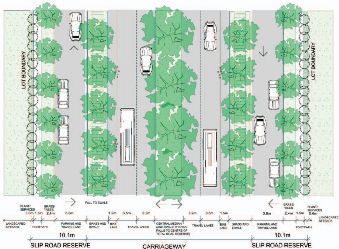
Plan - Major Rd (with Slip Rd)
