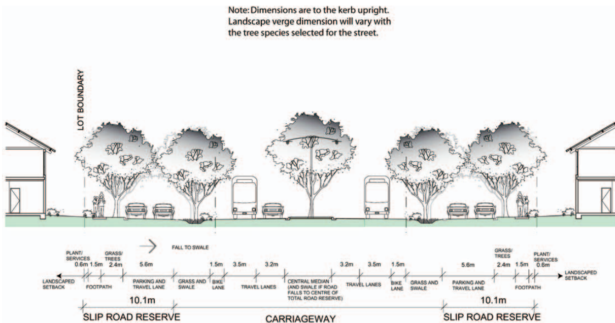
Section - Major Road (with Slip Rd)
