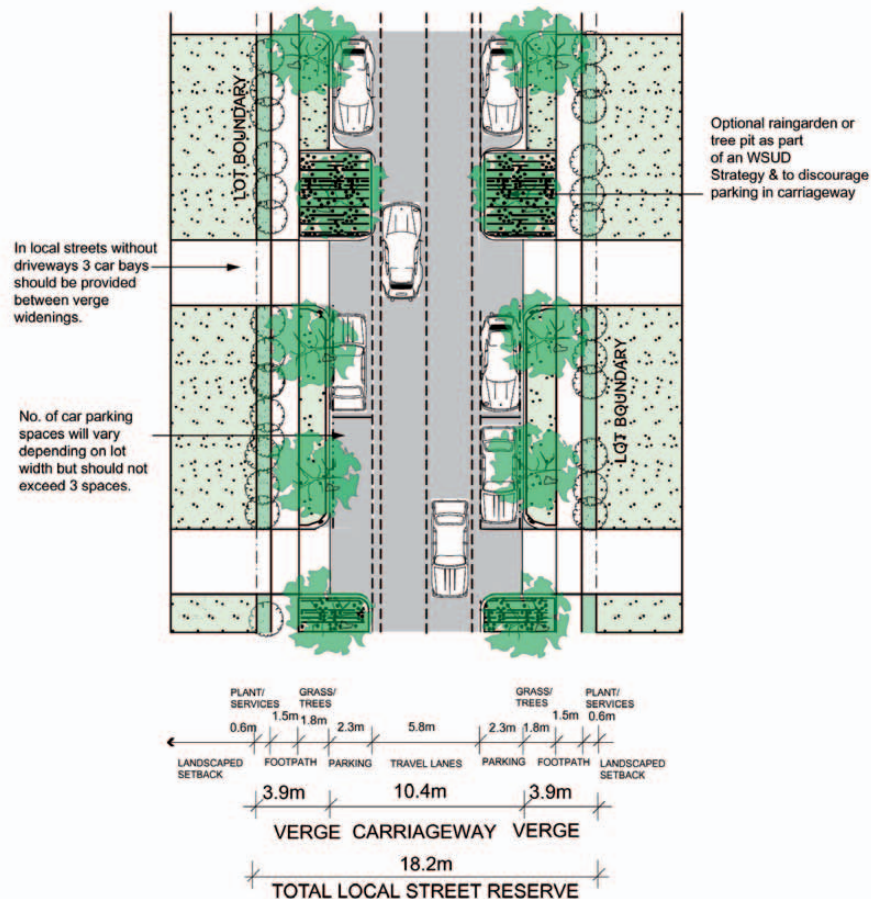
Plan - Local Street with inset parking bays (optional raingardens)
